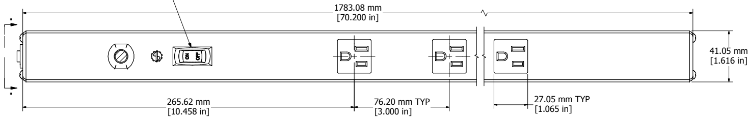
SECTION A-A (VIEW FROM FRONT)
