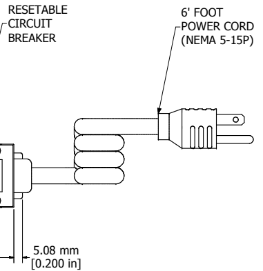
ASSEMBLY - VIEW FROM END
